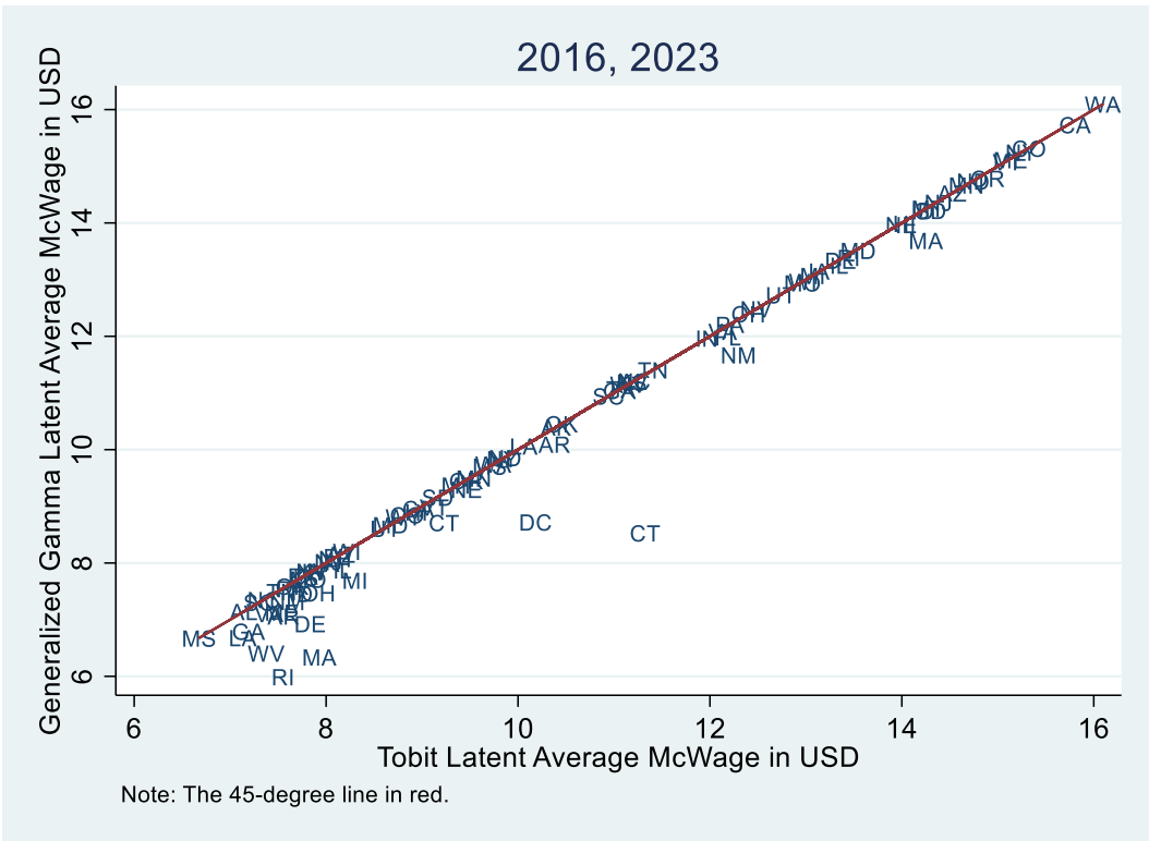
Fig. D.2: Latent McWage means based on the Normal distribution vs. the Generalized Gamma distribution Note: State-year data from 2016 and 2023.
