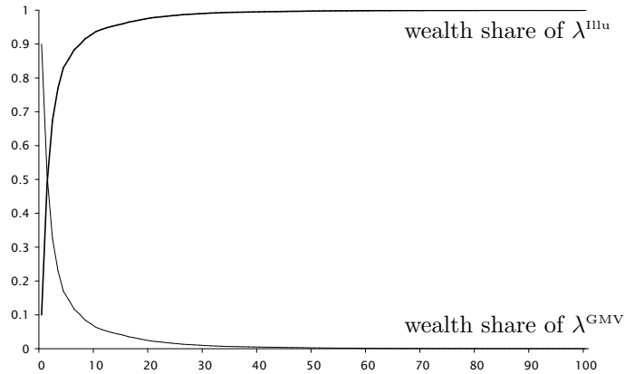
Figure 4: Dynamics of wealth shares in a market with an illusionary diversification strategy \lambda^{\text{illu}} and the globally minimum mean-variance rule \lambda^{\text{GMV}} .
